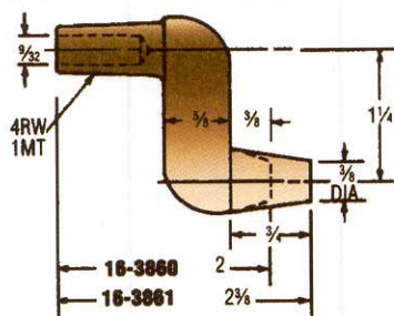
CMW ® 3 FORGED
