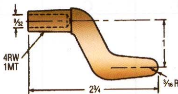
16-3837 CMW ® 3 CASTING
